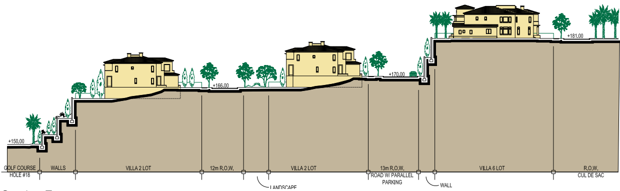
Section E
